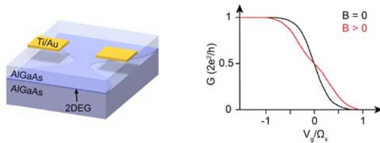
Quantum point contact structure (left) in which an applied voltage constricts electron movement to one dimension, with conductance (right) showing effect of applied magnetic field (red).
