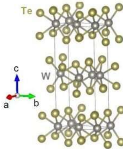
Model of tungsten ditelluride WTe 2 crystals in a layered, orthorhombic structure. Credit: FLEET
